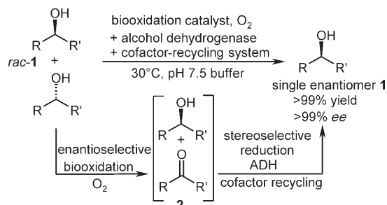
Scheme 1. Tandem biocatalysis for the deracemization of racemic secondary alcohols through an oxidation–reduction sequence.
